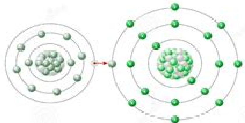
Ionic bond
