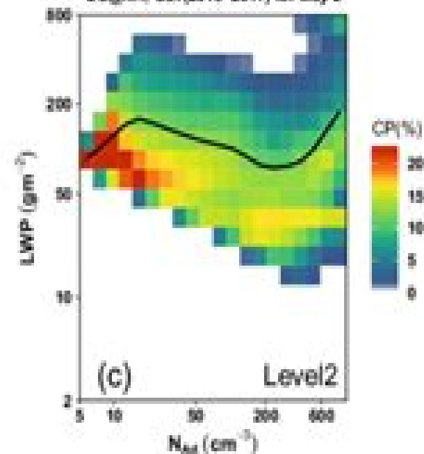
OC@GBL; CLY(2003-2020) for May 2
