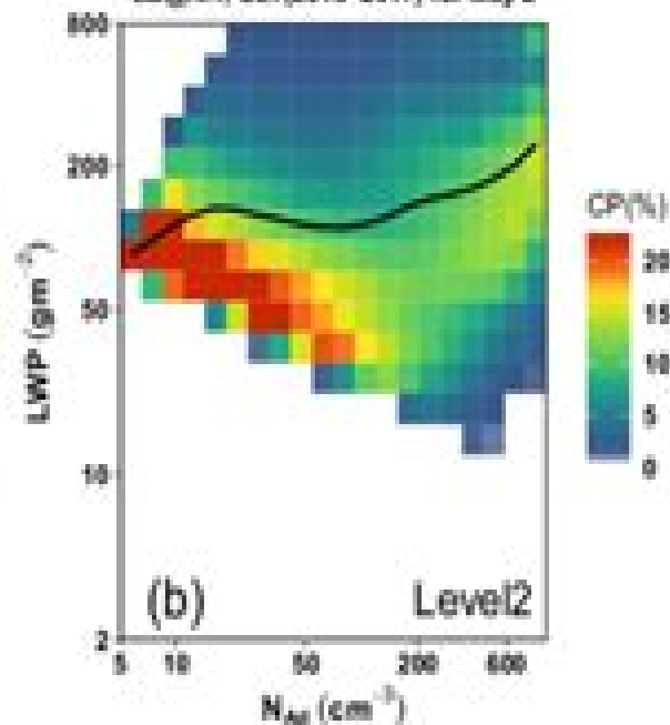
OC@NH; CLY(2003-2020) for May 2
