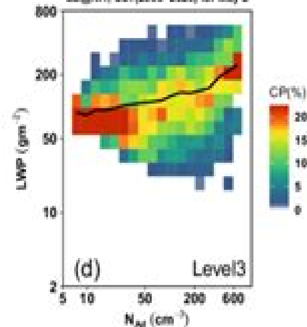
LD@NH; CLY(2003-2020) for May 2
