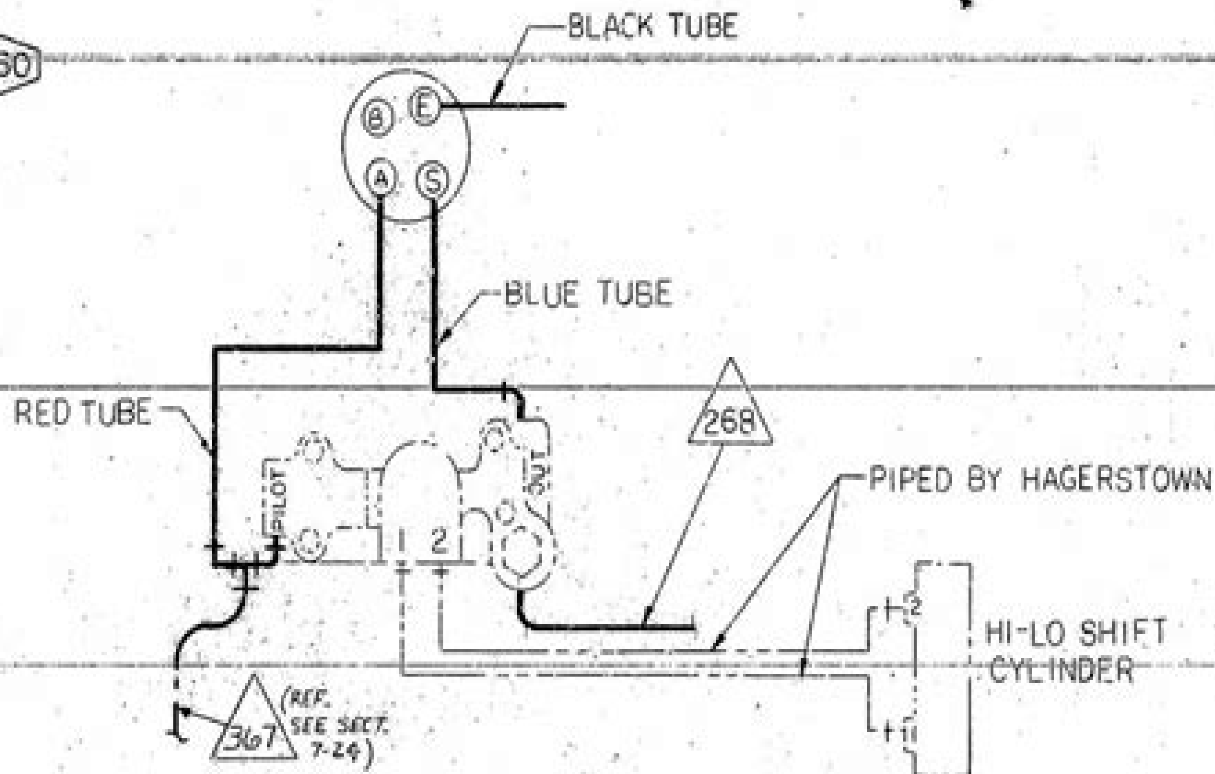
AIR CONTROL SCHEMATIC T2090 & T2100 TRANSMISSION
