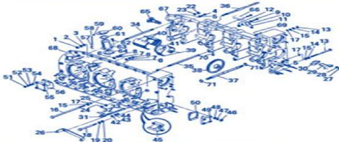
Figure 13. Exploded View of Typical Crankcase Assembly
