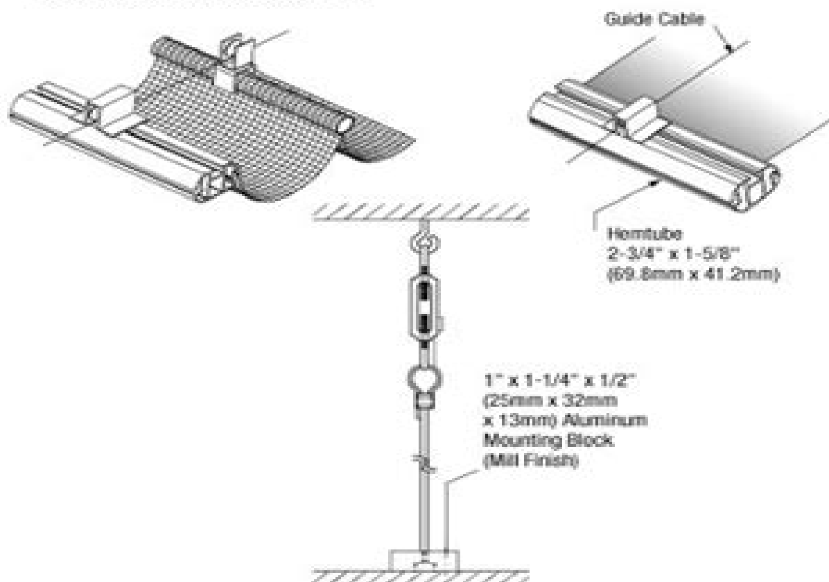
GP Hemitube with Guide Cable Detail
