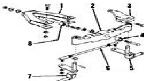
Fig. G10 — Exploded view of front axle assembly used on all models
