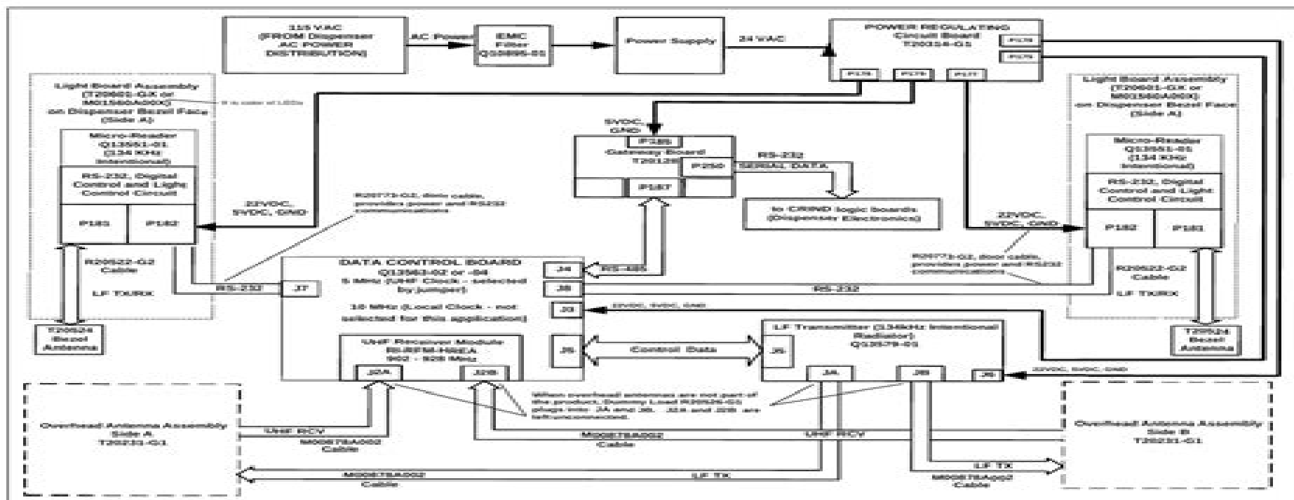
Figure 3-2: The Advantage Series Full System Block Diagram
