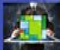
Operating System
