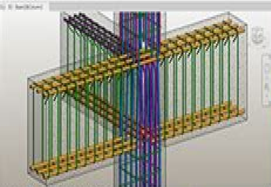
Fig. 10: Reinforcement
