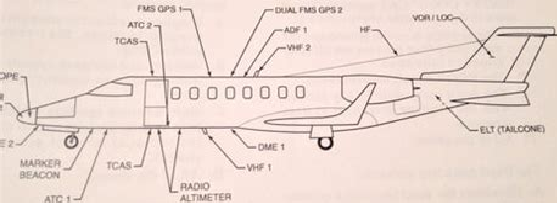
Figure 1-21. Airplane Antennas
