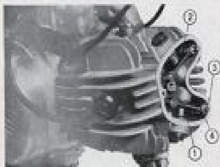
FIGURE N° 7 - Adjustment of rocker arm clearance 1. exhaust-arm driving exhaust valve 2. inlet rocker-arm driving inlet valve 3. adjusting screw 4. lock nut
