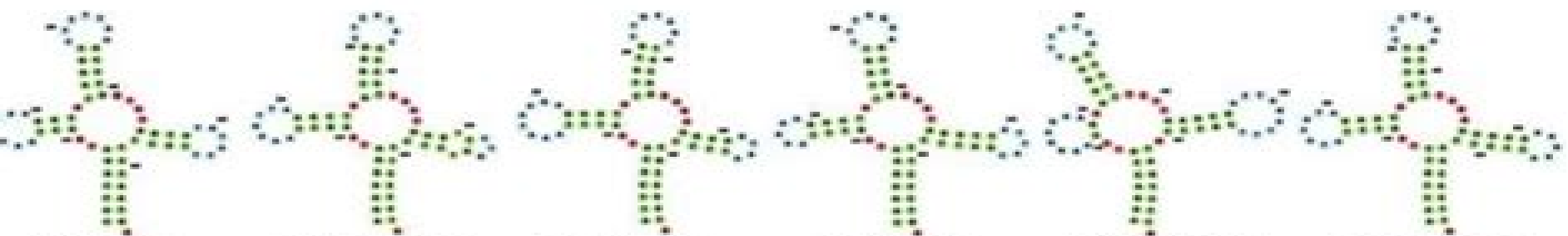
tRNA - Lys
