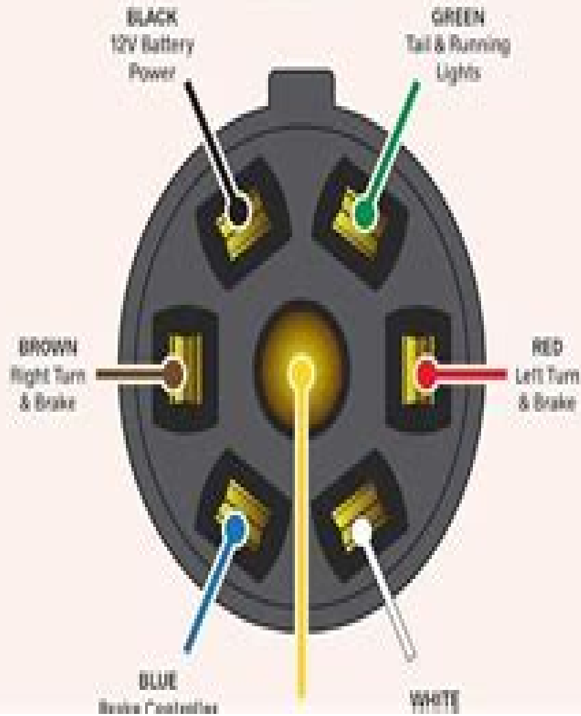
Plug Side
