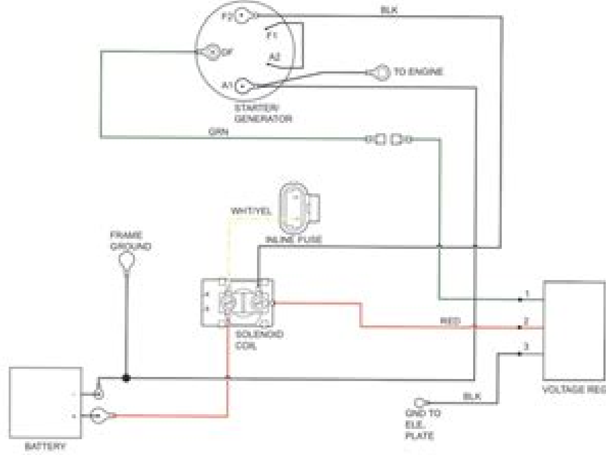
Fig. 2 Electrical System Wiring Diagram
