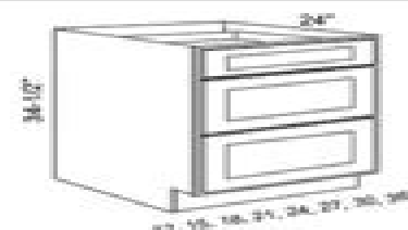
3-Drawer Bases DB12-3, DB15-3, DB18-3, DB21-3 DB24-3, DB27-3, DB30-3, DB36-3
