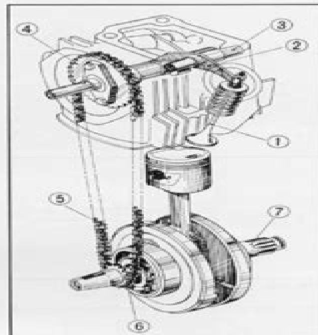
Fig. 3. 28 Valve mechanism ① Valve ② Rocker arm ③ Rocker arm shaft ④ Cam sprocket ⑤ Cam chain ⑥ Timing sprocket ⑦ Crankshaft
