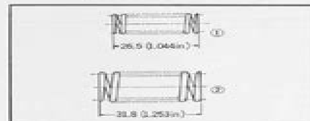
Fig. 3. 29 Valve spring ① Inner spring ② Outer spring
