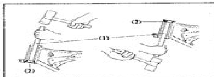
Fig. 5-67 (1) Ball race remover (2) Ball race
