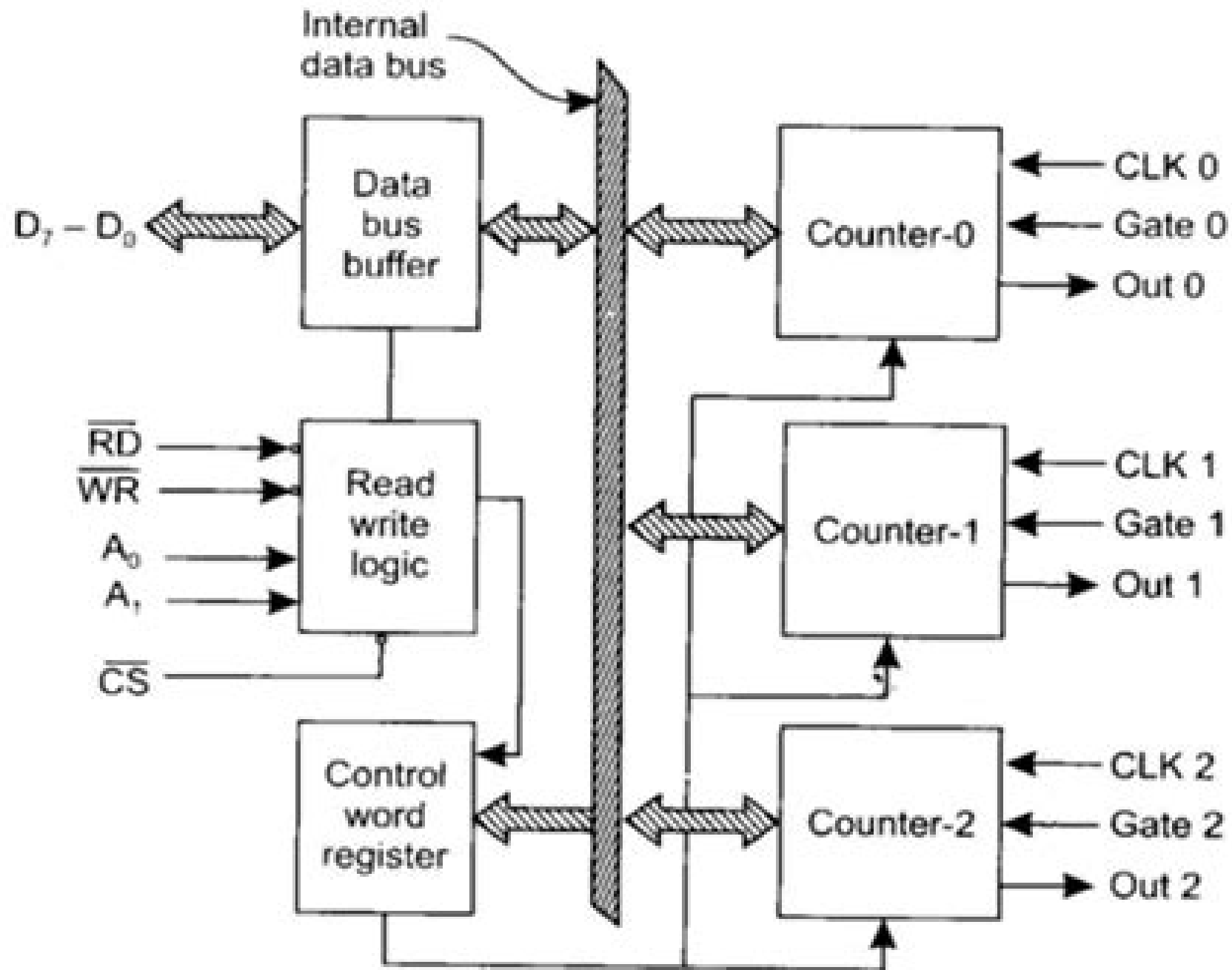
Fig. 9g.2: 8253 Functional block diagram (Source: Intel Corporation)
